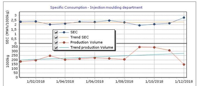
Evolution of the Specific Energy Consumption (SEC) in combination with the production output. Decreasing SEC does not necessarily mean that the plant is operating more energy efficient; it can also be the result of a higher production volume, resulting the base load to be divided over a higher output volume.
