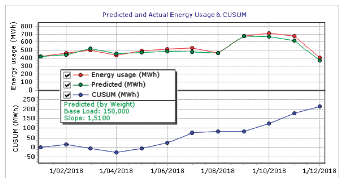
CUSUM chart with actual and target consumption. In case actual consumption is in line with target, the cumulative deviations should be scattered around zero. Deviations from target result in rising (actual consumption higher than target) or falling (actual consumption lower than target) CUSUM charts.
