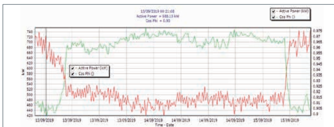
Electricity consumption and power factor during the weekend.
