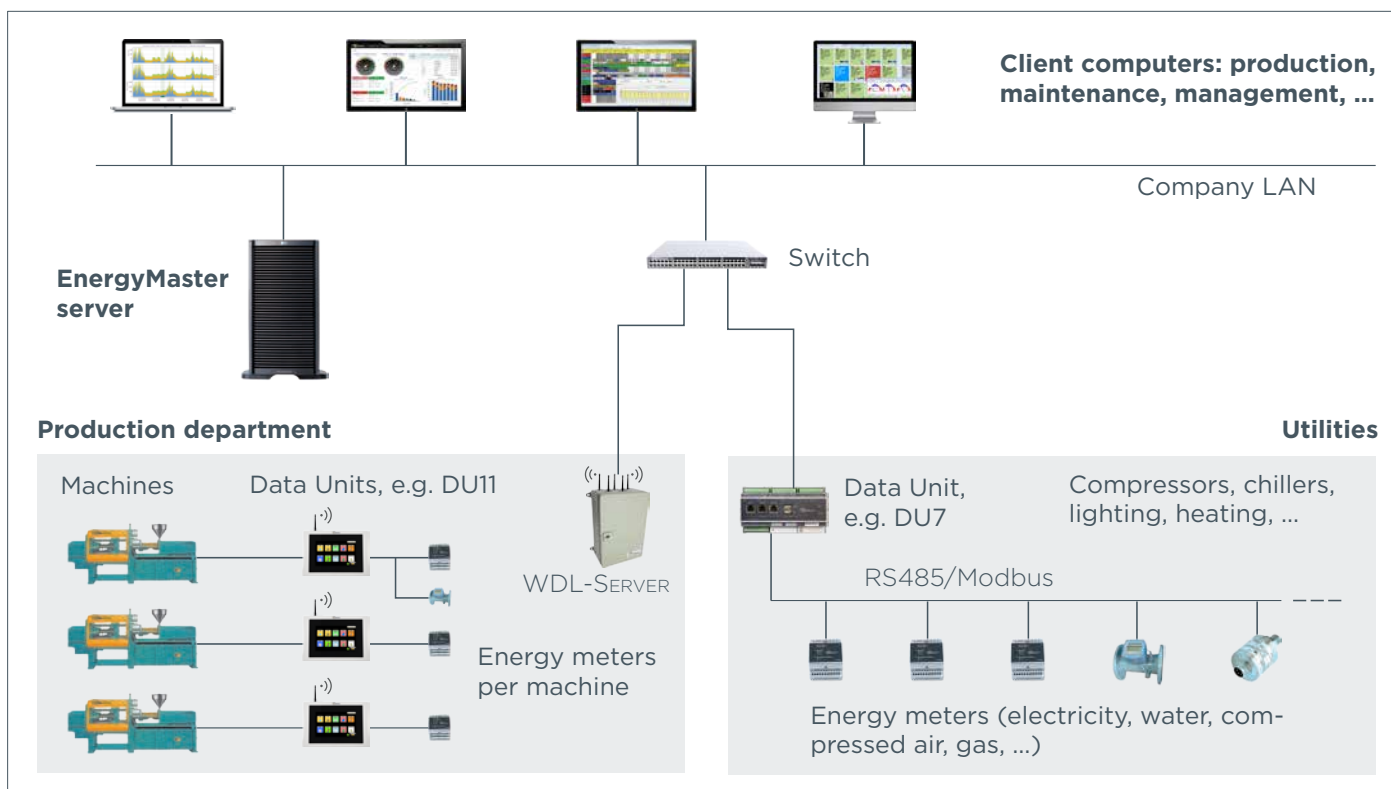
ENERGYMASTER concept. Existing BMSvision Data Units can be used to collect the meter counters. This data is transferred to the ENERGYMASTER server over the existing BMSvision network (wired or wireless). For new installations, a wireless network is the best choice.
